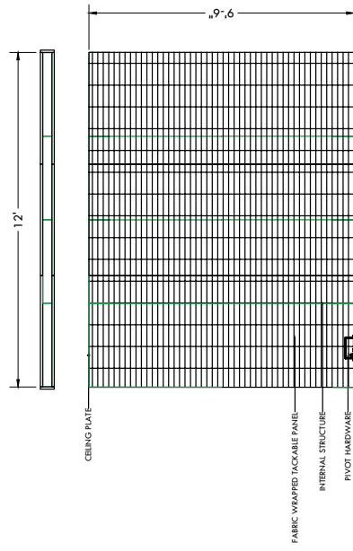
5 ELEVATION E SCALE: 1/4" = 1'-0" Pivoting Walls Overall 114" x 144" Individual Panels 114"x 47 5/8"
